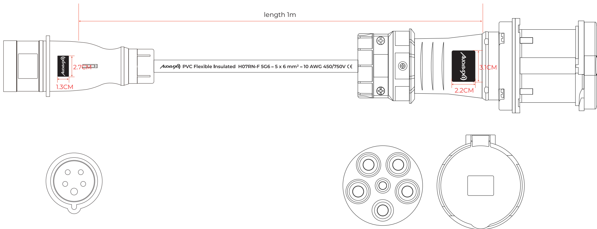
32A CEE 5-pin M
