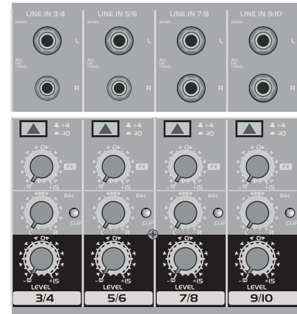
Fig. 2.2: Connectors and controls on the stereo channels
