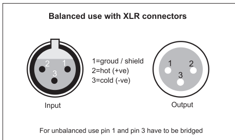
Fig. 4.1: XLR connections
